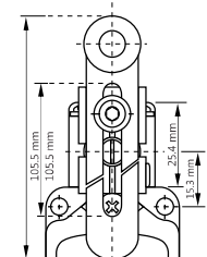
Adjustable Roller Lever
