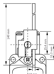
Adjustable Rod Lever
