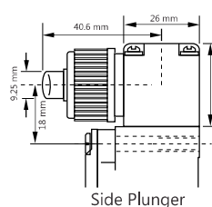
Side Plunger
