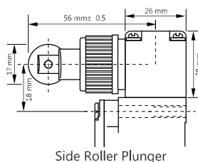
Side Roller Plunger
