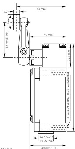
Roller Lever
