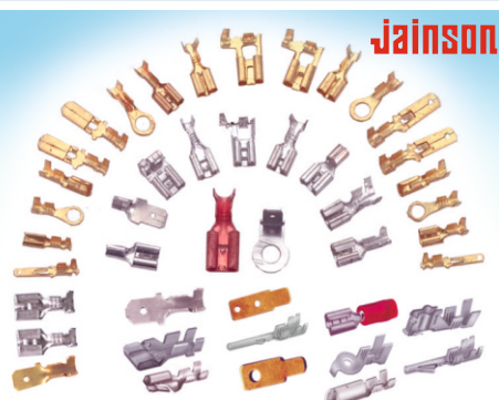
SNAP ON TYPE TABS
